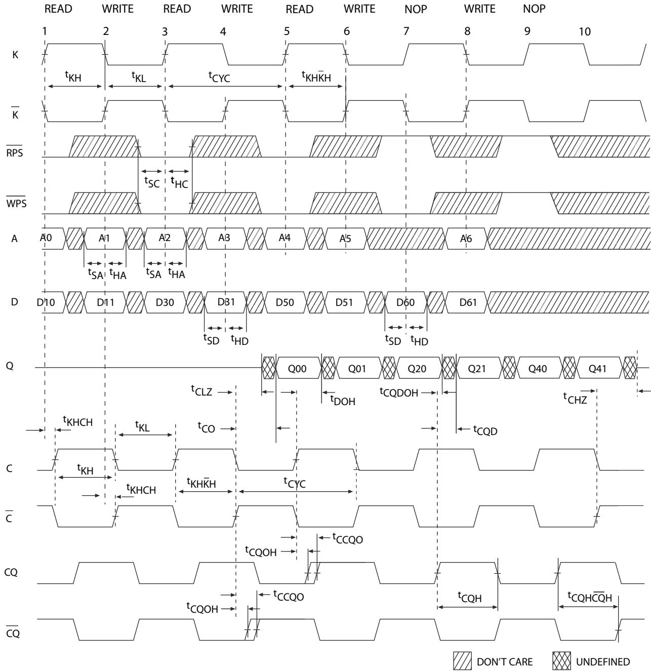
Figure 5. Read/Write/Deselect Sequence [36, 37, 38]
